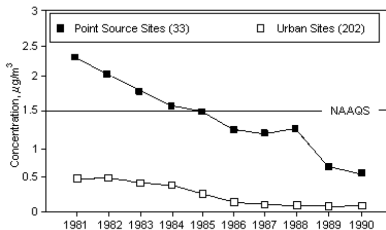
Fig. 3. Comparison of national trend (USA) in the composite average of the maximum quarterly lead concentrations at urban and point source oriented sites, 1981-1990 (NAAQS=National Ambient Air Quality Survey). (From: US EPA, 1991)
