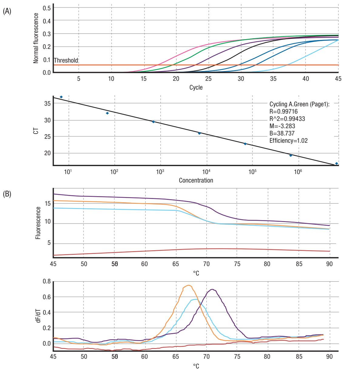
Figure A3.3 (A) Typical real-time PCR amplification curves showing specimens with a serial dilution of target DNA and the standard curve; (B) Melting curve analysis using melting temperatures ( T_m ) to enhance the specificity of SYBR Green-based real-time PCR.
